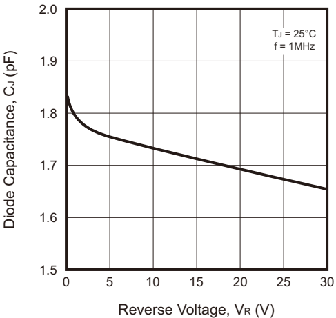
Fig.2 - Capacitance Characteristics
