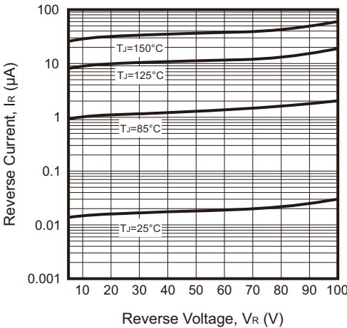
Fig.4 - Reverse Characteristics
