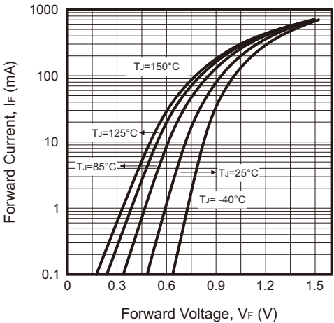
Fig.3 - Forward Characteristics
